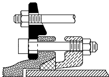
SDR 26 INSTALLATION
